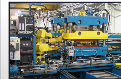
APS System with In-line Robotic Welding
