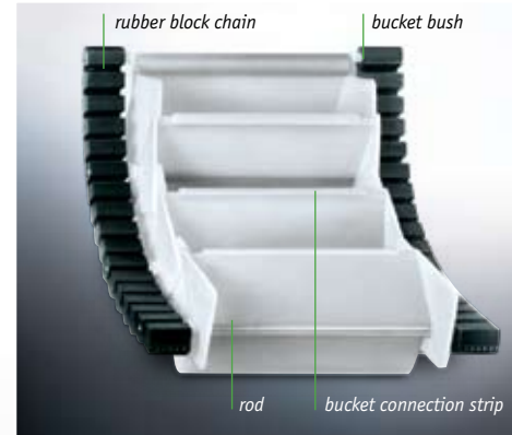
Bucket belt components and rubber block chain
