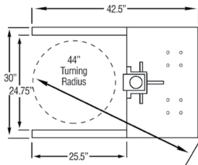
Base for Straddle Roto-Grip™
