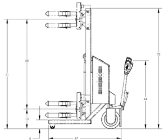
Straddle Power Drive Roto-Lift®
