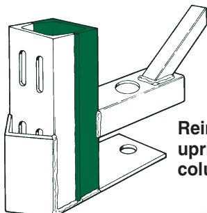
Structural angle pallet support
