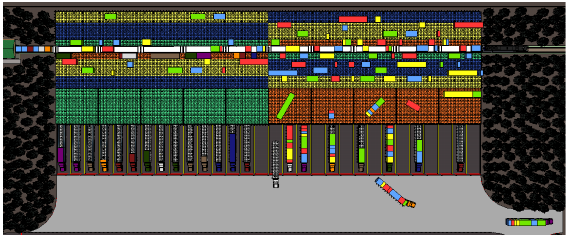
Figure 21: Train stopped with first railcars in unloading positions.
