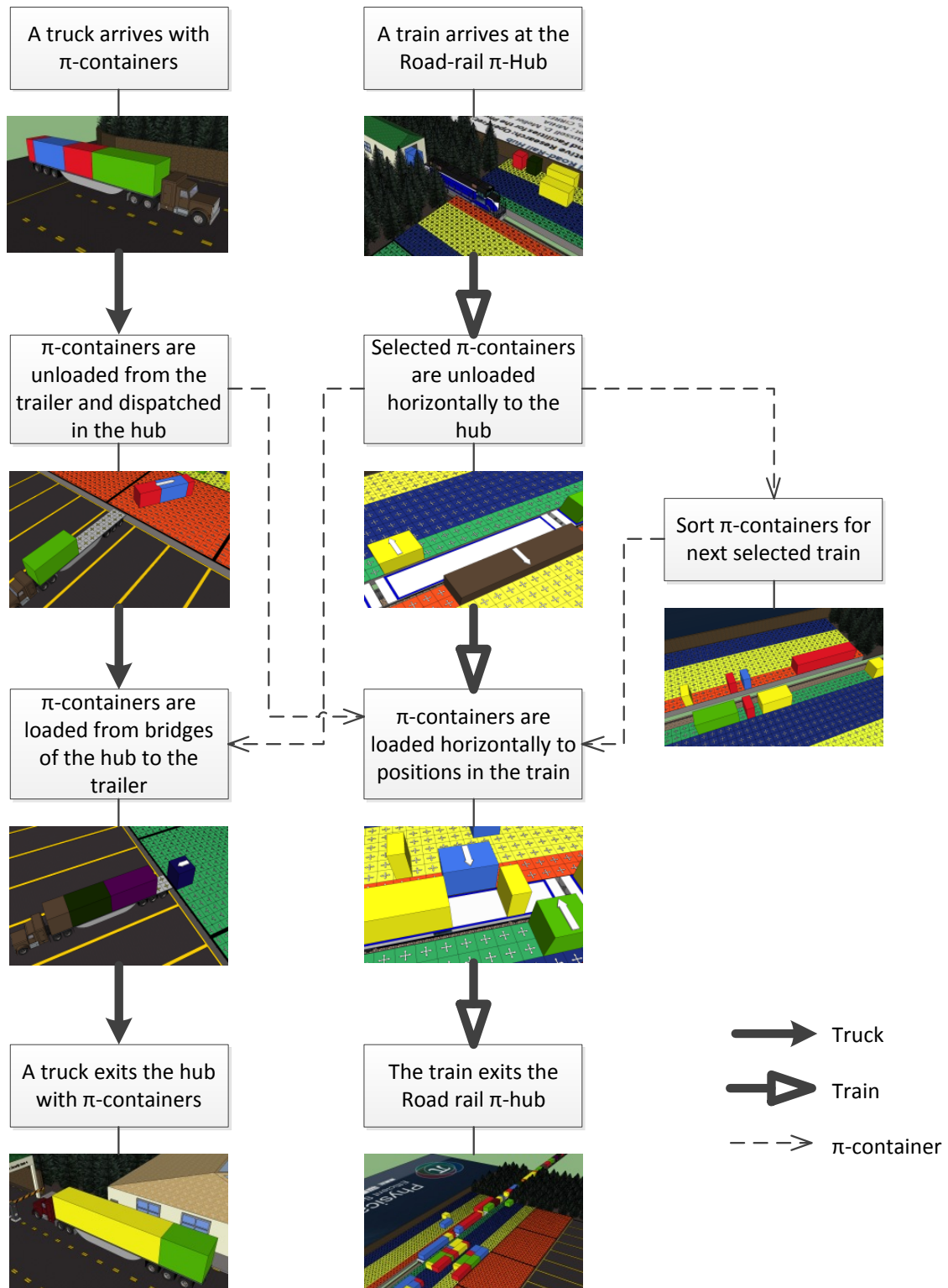
Figure 2: Overview of the flow of trucks, trains and \pi -containers in the road-rail \pi -hub
