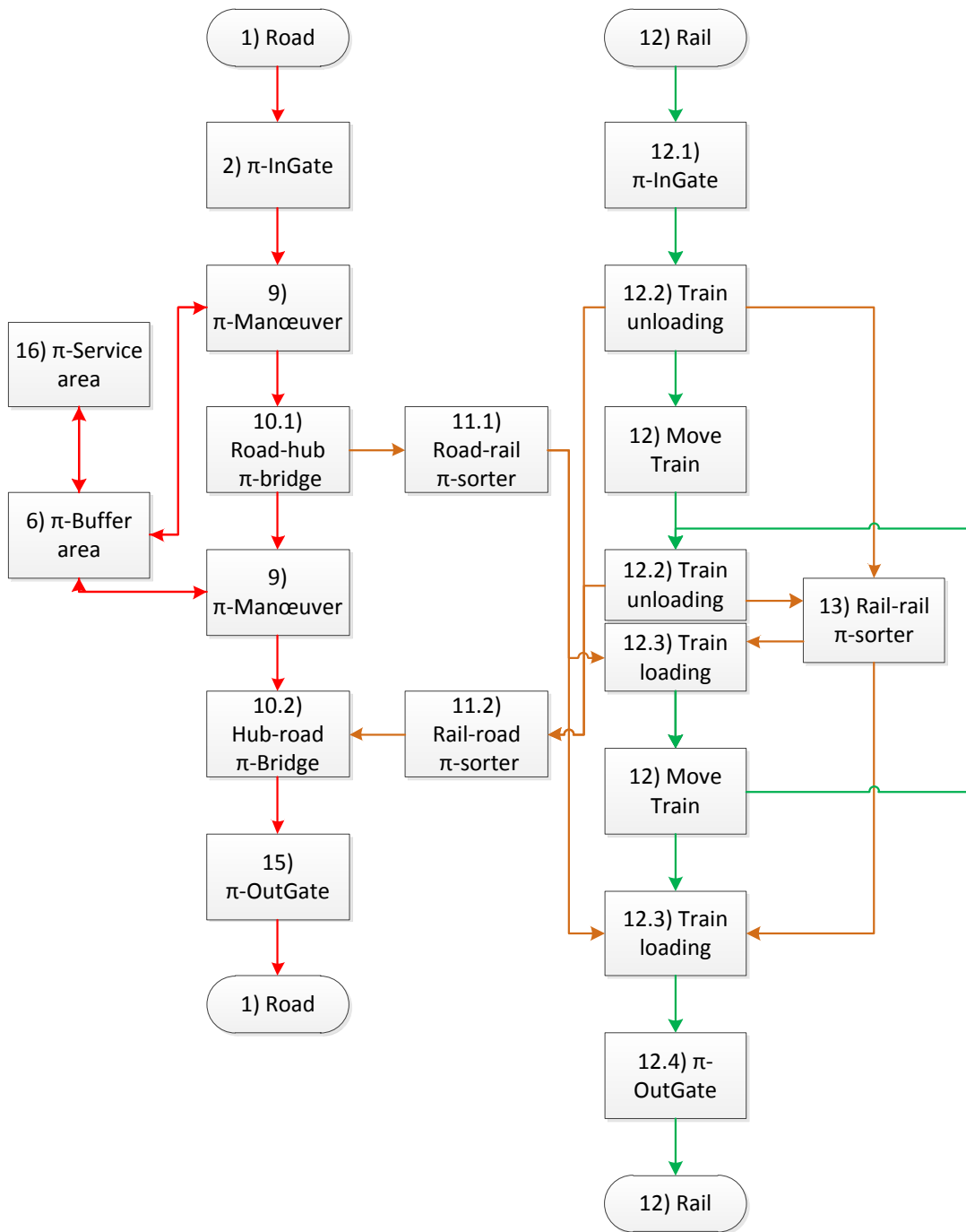
Figure 5: Illustration of the Major Flows in a Road-Rail \pi -Hub
