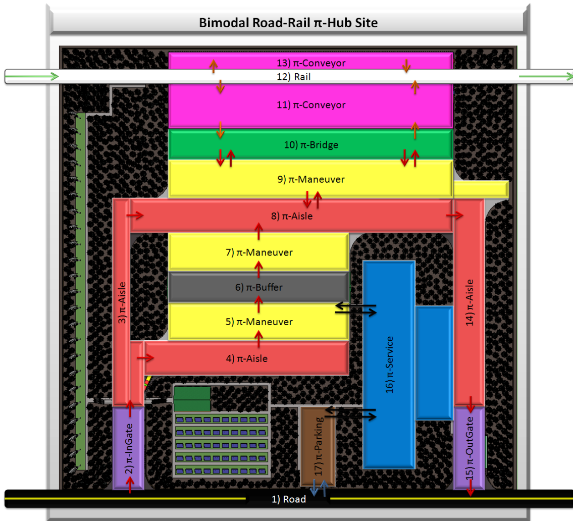
Figure 7: Block Layout for the Proposed Functional Design.
