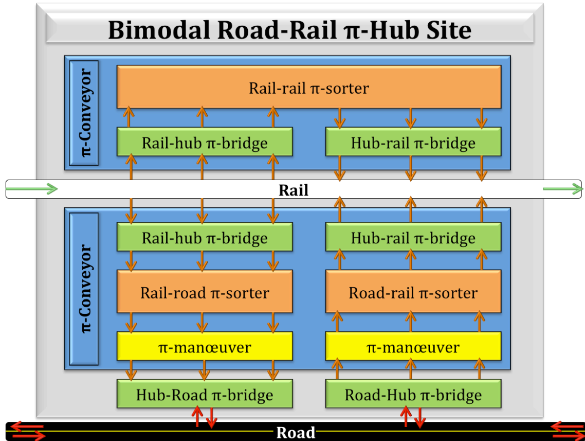
Figure 6: Proposed Functional Design of the Road-Rail \pi -Hub
