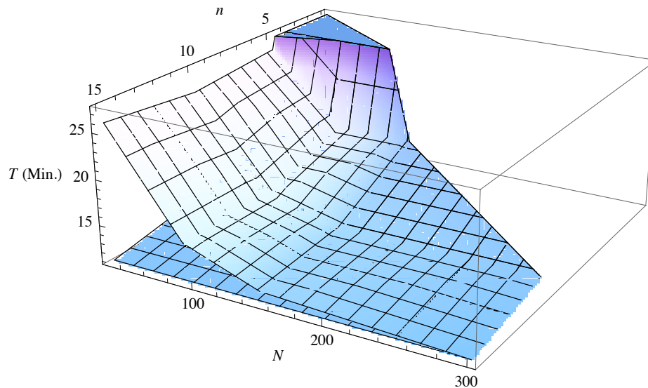
Figure 8: Process time T according to p=1 (complete unload and reload of the train in the hub) where the higher surface represents T according to s_{1,2}=1 (highest amount of handling) and the lower surface according to s_{1,2}=1 (smallest amount of handling)
