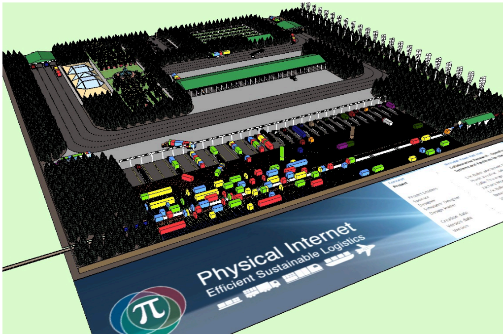
Figure 10: Final Layout of Proposed Design (Rear View)
