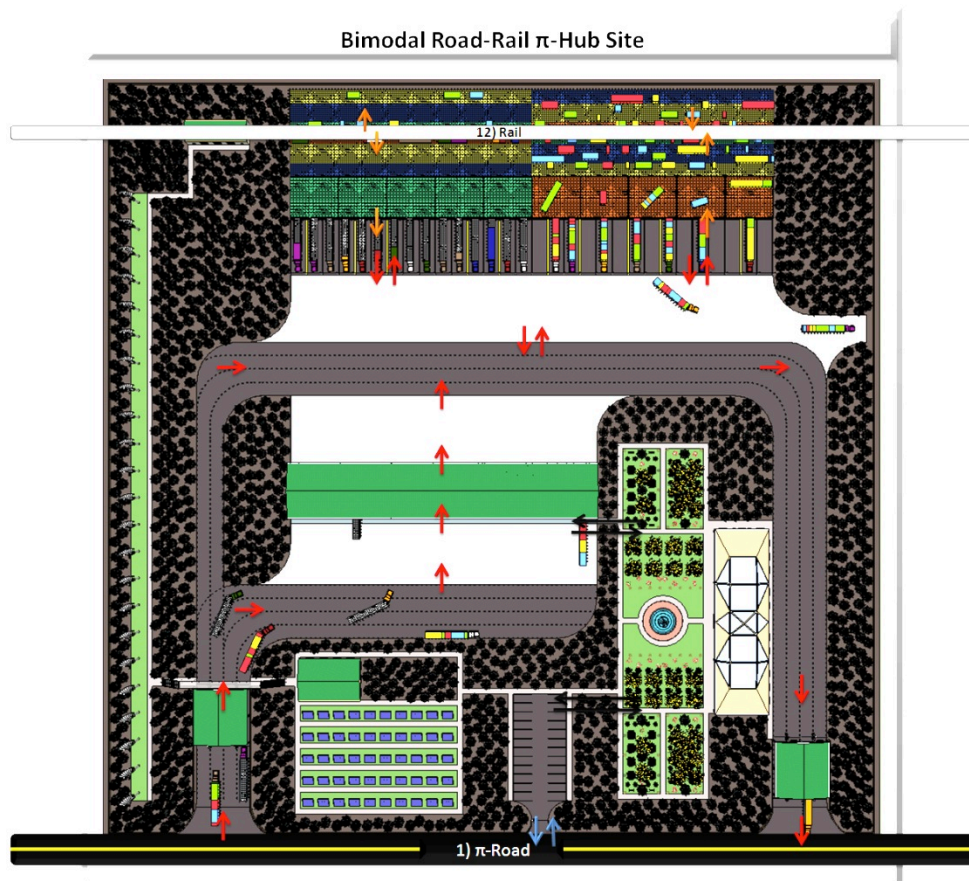
Figure 9: Final Layout of Proposed Design (Overhead View)
